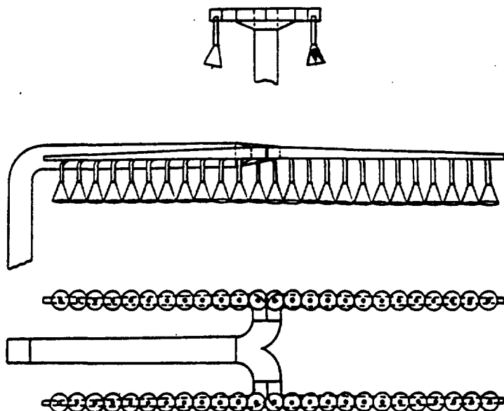
FIGURE 2.—Schematic views of exhaust system applied to Foster winders.
