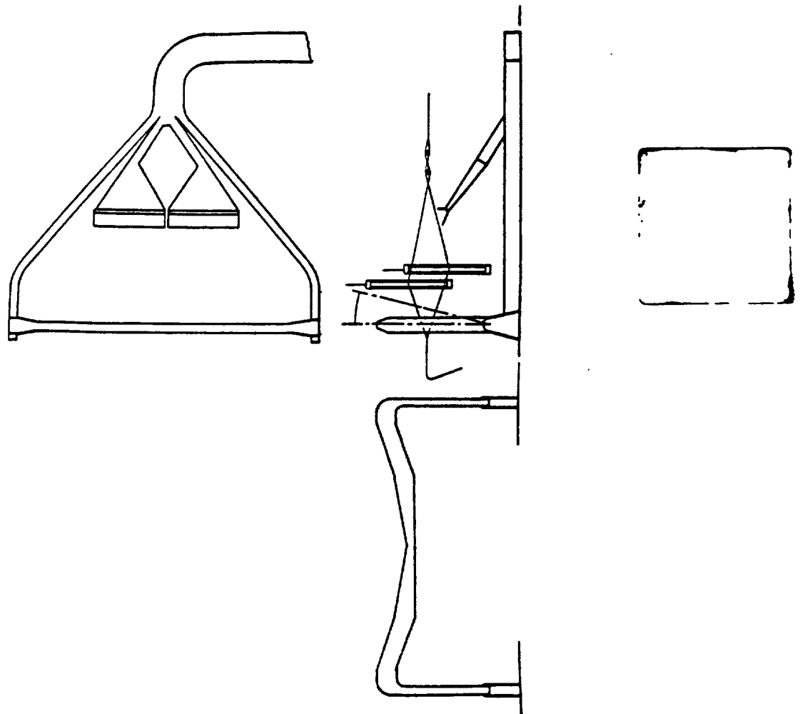
FIGURE 11.—Schematic views of exhaust system applied to broad looms.
