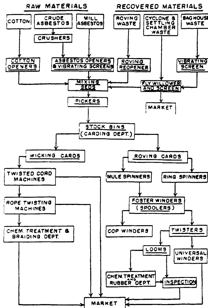
FIGURE 1.—Process flow-chart, asbestos textile plant.
