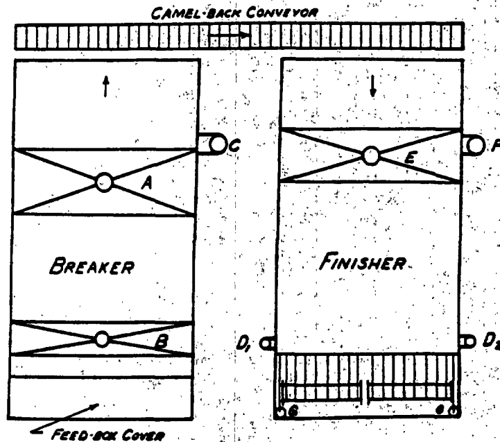
FIGURE 7.—Schematic plan of card exhaust system.
