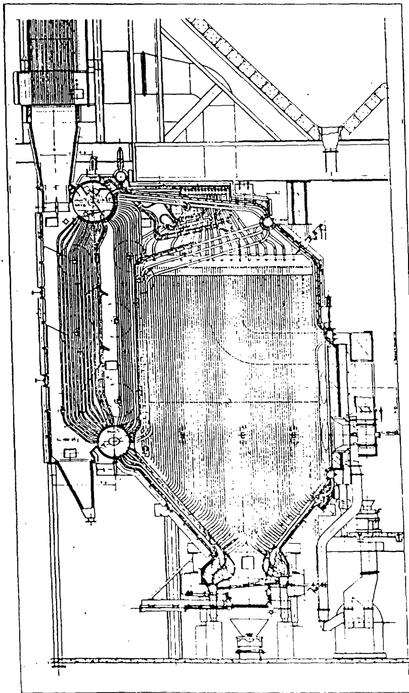
UNION ELECTRIC COMPANY OF MISSOURI, 2-285,000 pounds per hour, 250 pounds pressure,
