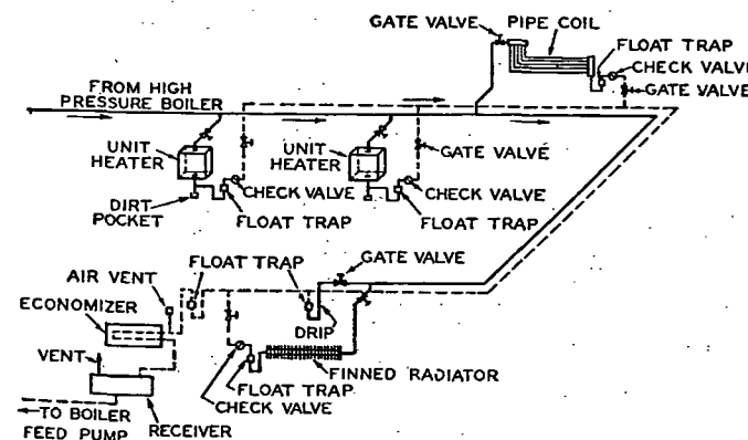
FIG. 9. TYPICAL HIGH PRESSURE HEATING SYSTEM
