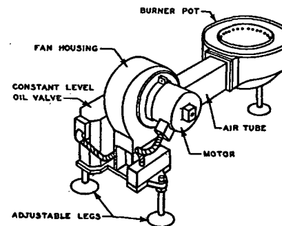
FIG. 15. VAPORIZING FORCED-DRAFT POT-TYPE BURNER
