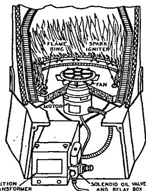
FIG. 14. WALL FLAME VERTICAL ROTARY BURNER
