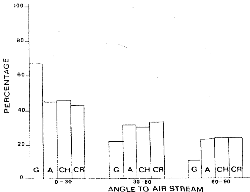
Figure 3: Frequency histograms in which percentage of fibres is plotted against angle to the airstream (axis of duct) in the aerosol spectrometer, for glass, amosite, chrysotile and crocidolite fibres with aspect ratios > 5 .
