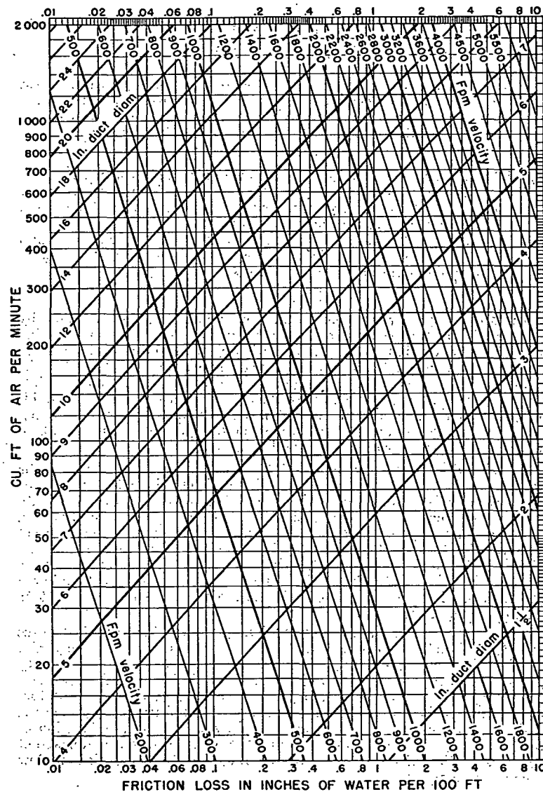
FIG. 1. FRICTION OF AIR IN STRAIGHT DUCTS
