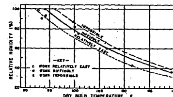
Fig. 3 . . . Heat Endurance of Acclimatized Subjects Working at a Specific Rate 10
