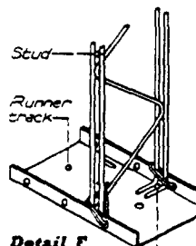
Detail F Bend one or both legs of stud to form shoe which is wired to runner track.
