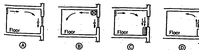
FIG. 16. DISTRIBUTION METHODS FOR SMALL ROOMS
