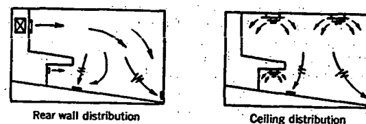
FIG. 15. AIR DISTRIBUTION METHODS FOR THEATERS, CHURCHES, AND AUDITORIUMS
