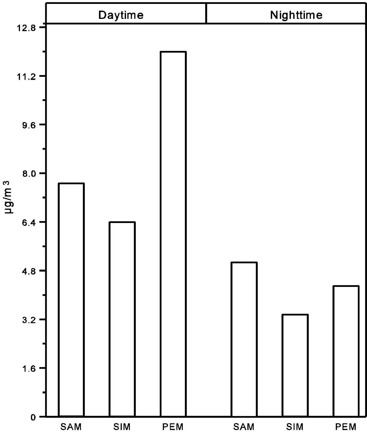
Figure 3-3. Mean outdoor stationary ambient monitor (SAM), stationary indoor monitor (SIM), and personal exposure monitor (PEM) silicon (<10 \mu\text{m} particle size) concentrations for 178 residents of Riverside, CA.
