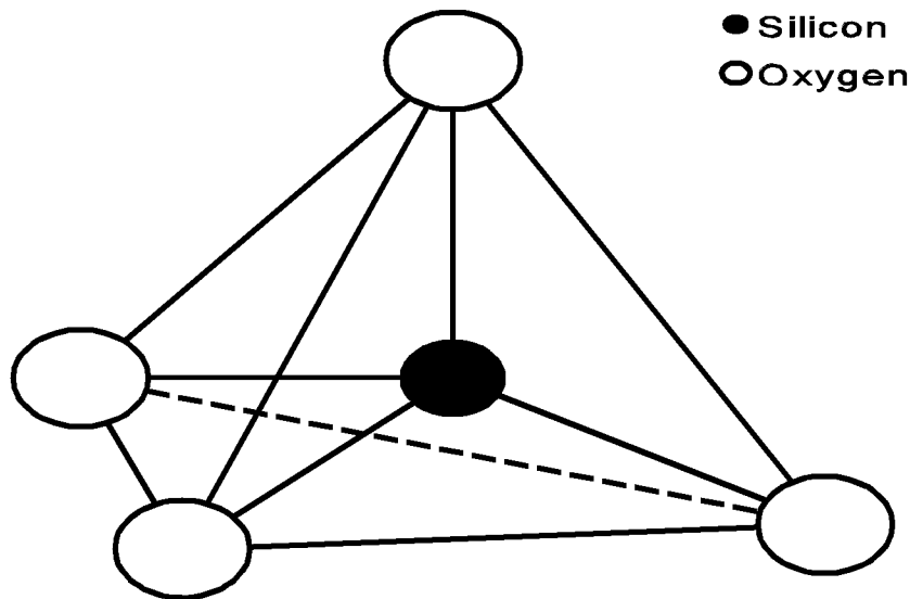
Figure 1-1. Silicon-oxygen tetrahedron.
