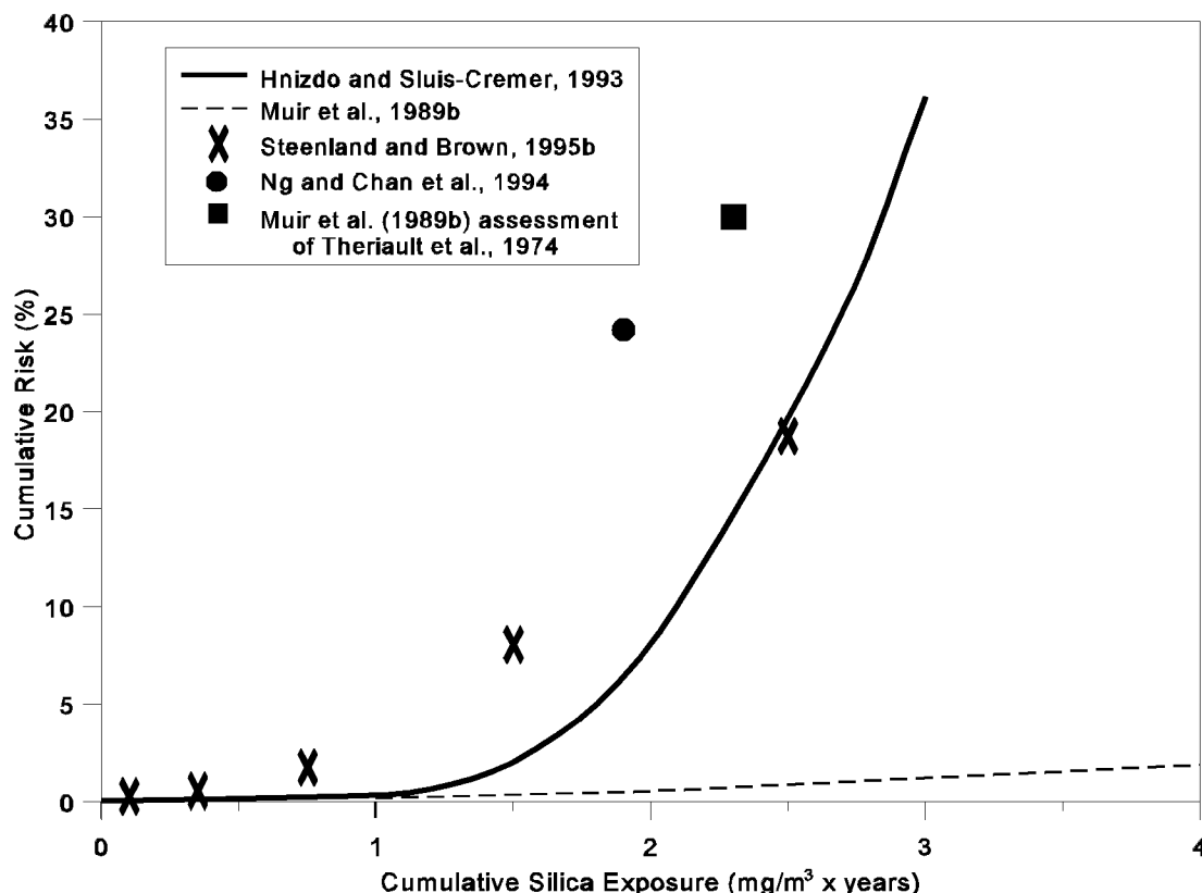
Figure 7-1. Cumulative silica risk curves estimated for South African gold miners (—) (Hnizdo and Sluis-Cremer, 1993) and Canadian hardrock miners (---) (Muir et al., 1989b); cumulative silica risk points estimated for South Dakota gold miners (X) (Steenland and Brown, 1995b), Hong Kong granite workers (●) (Ng and Chan, 1994), and Vermont granite miners (■) (Theriault et al., 1974c; Muir et al., 1989b).
