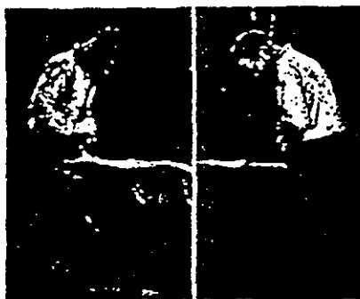
Figure 2. Left: Operator in monument shed using pneumatic hammer. Neither dust control nor respirator has been provided. Right: The same operation with goggles and dust-control hood in use.
