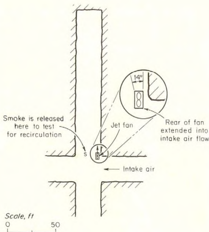
Figure 1. Jet fan ventilating a straight single heading.
