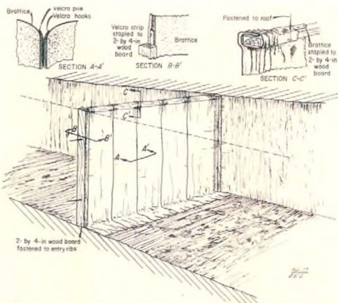
Figure 5. Stopping constructed from damage-resistant brattice.
