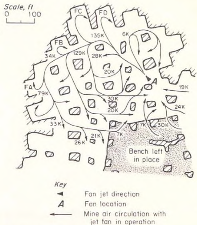
Figure 4. Airflows obtained with jet fan in operation.
