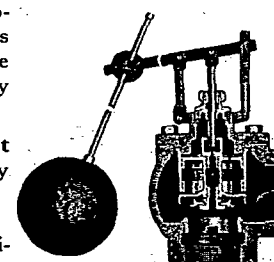
No. 7 Single Seated Float Valve
