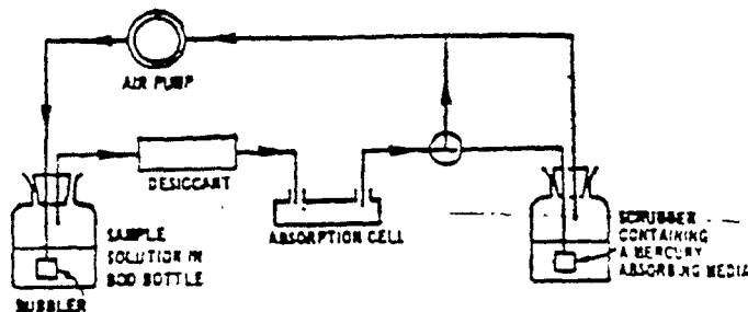
Figure 105-1. Apparatus for flameless mercury determination.
