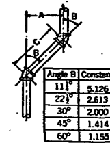
FIG. 38. CONSTANTS FOR DETERMINING LENGTH OF OFFSET PIPE
