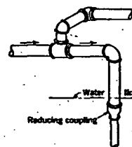
FIG. 34. DRIPPING MAIN WHERE IT RISES TO HIGHER LEVEL
