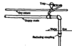
FIG. 40. DRIPPING END OF MAIN INTO WET RETURN
