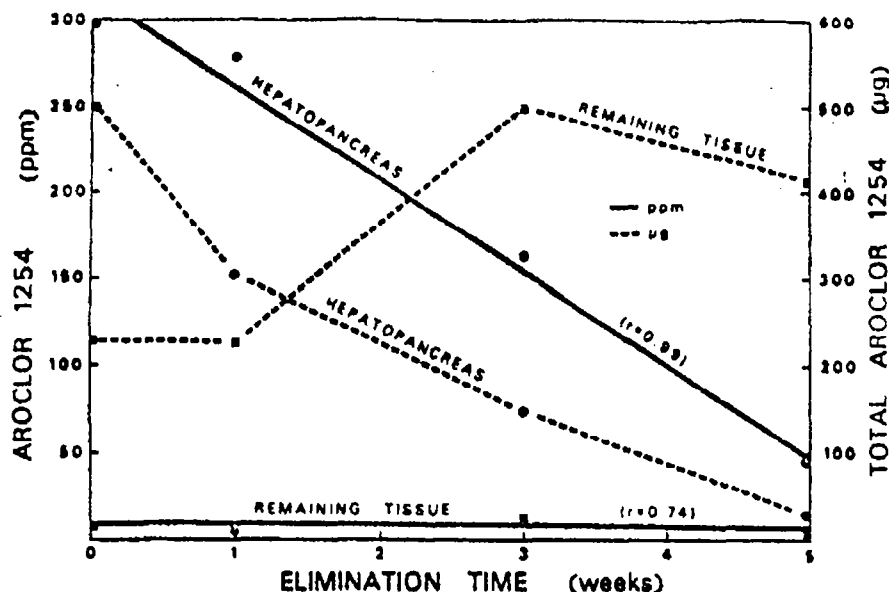
Fig. 5. Penaeus duorarum . Rates of elimination from hepatopancreas and subsequent increase in remaining tissue. Shrimp were exposed to 7.5 ppb Aroclor 1254 in flowing water for 16 days, then placed in Aroclor-free environment. Composite tissue samples from 8 individuals were analyzed for each determination. Unexposed shrimp showed no detectable residues. r = correlation coefficient
