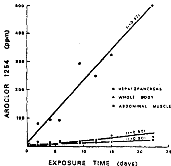
Fig. 4. Penaeus duorarum . Rates of absorption of Aroclor 1254, in various tissues of shrimp exposed to 2.5 ppb of the chemical in flowing water. Unexposed shrimp showed no detectable residues. r = correlation coefficient
