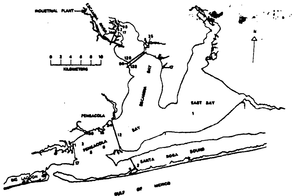
Fig. 1. Residues of Aroclor 1254 (in ppm) found in shrimp hepatopancreases from Escambia Bay and contiguous waters during 1969/1970. Each sample listed represents composite tissues of at least 5 individuals
