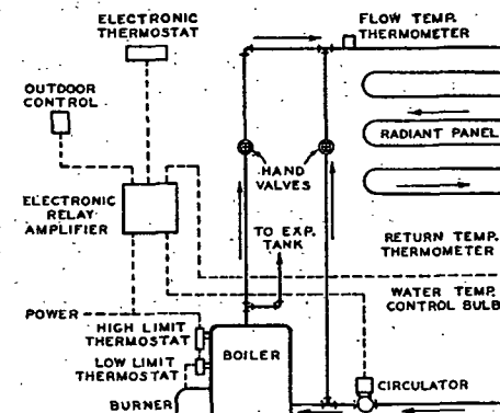
FIG. 4. ELECTRONIC CONTROL SYSTEM FOR PANEL HEATING
