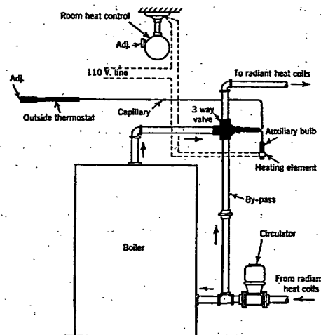
FIG. 3. PANEL HEATING CONTROL SYSTEM
