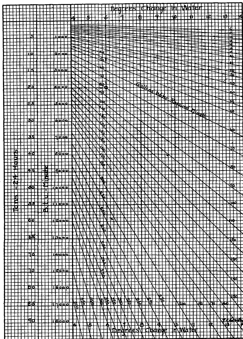
FIG. 78. GALLONS WATER REQUIRED PER MINUTE
