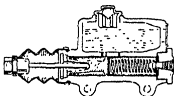
Figure 3 Integral Tank Type Master Cylinder
