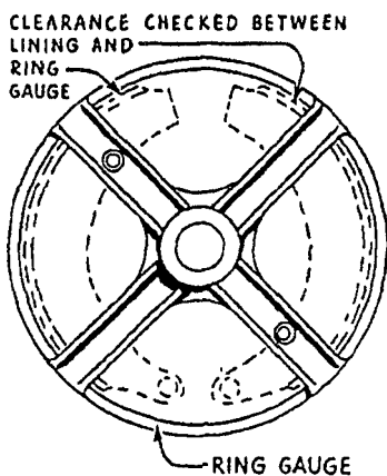
Figure 4 Ring Gauge in Place
