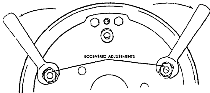
Figure 7B Method of adjusting eccentric cams on Lockheed Self adjusting Brakes
