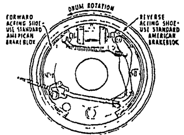
Figure 18 Chevrolet Huck Brake, Hydraulically Operated, Showing Mechanical Operation of Pear Brakes for Rarking
