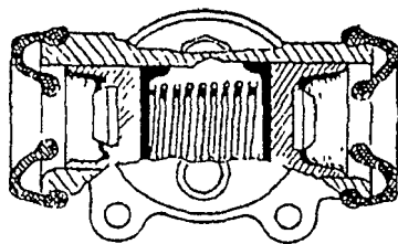
Figure 2 Wheel Cylinder
