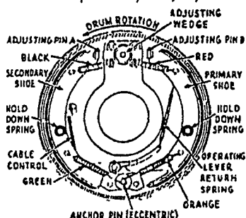
Figure 18 Ford Brakes (1937)—Left Front
