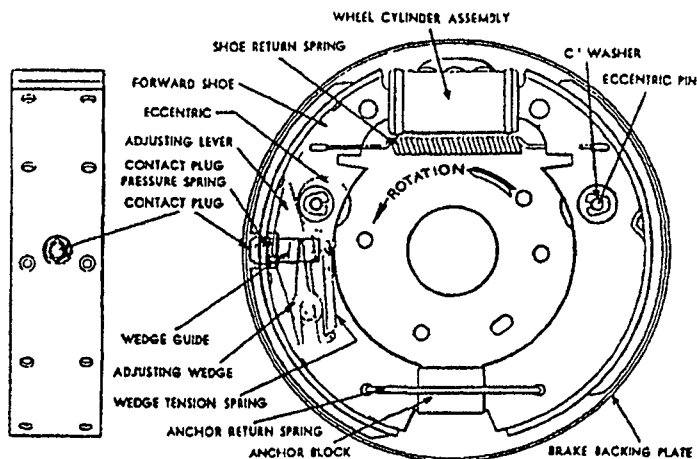
Figure 7A Lockheed Self-Adjusting Hydraulic Brake.
