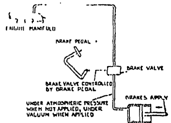
Figure 31 Layout of Atmospheric Suspended Vacuum Brake System (Single Line)
