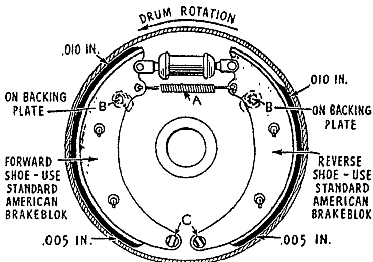
Figure 1 Lockheed Hydraulic Brake
