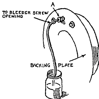
Figure 5 Method of Bleeding Hydraulic Brakes
