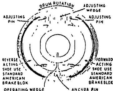
Figure 14 Ford Brake (1935-36) Left Front
