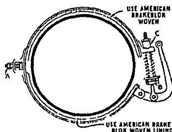
Figure 21 External Type Brakes Mechanically Operated
