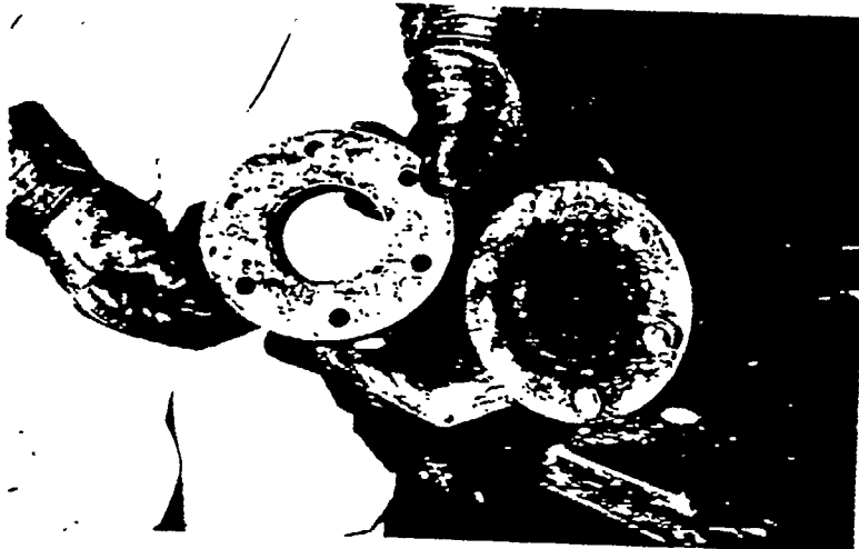
-Photo 4- Removed gasket. Fitting #58A is shown.
