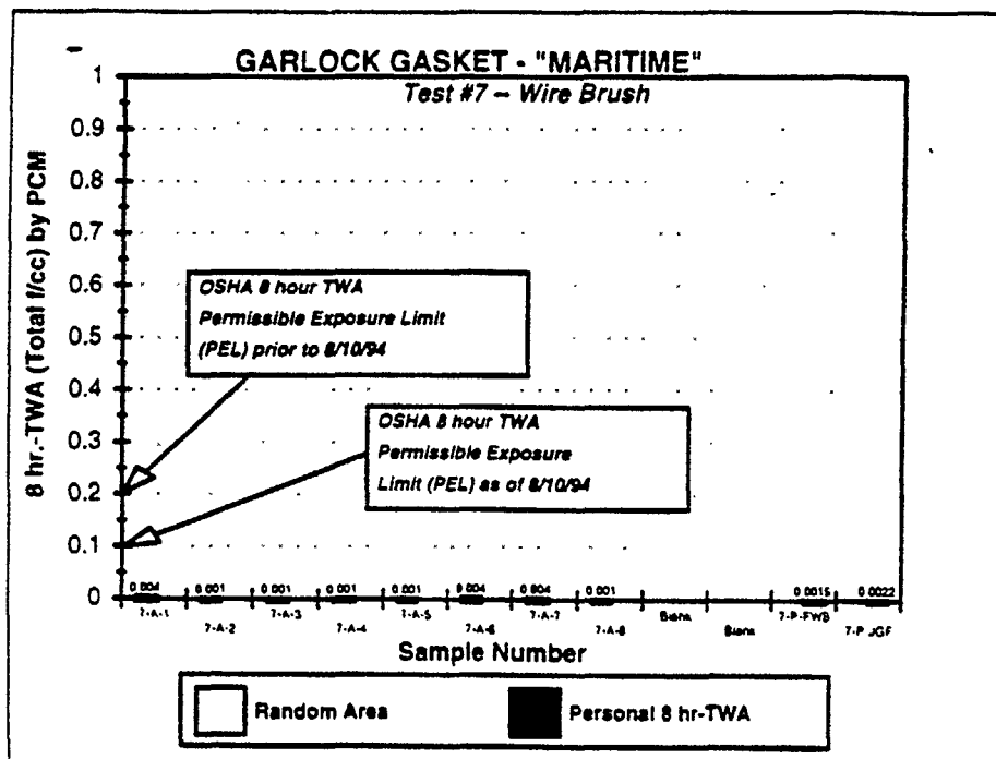
Figure 2 - Graphical presentation of air sampling results.
