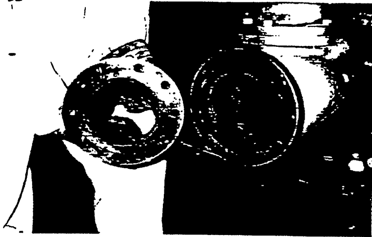
-Photo 7- Flange after "facing". Fitting #51B is shown.
