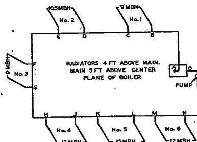
FIG. 11. ONE-PIPE FORCED CIRCULATION SYSTEM (EXAMPLE 4)
