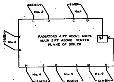
FIG. 10. ONE-PIPE GRAVITY CIRCULATION SYSTEM (EXAMPLE 3)
