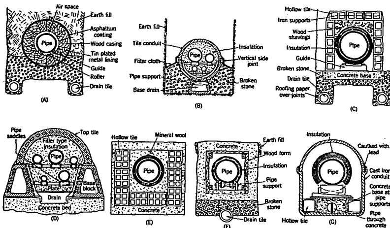
FIG. 1. CONSTRUCTION DETAILS OF CONDUITS COMMONLY USED
