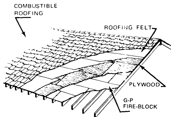
Plywood Sheathed Roof over G-P Fire-Block Gypsumboard
