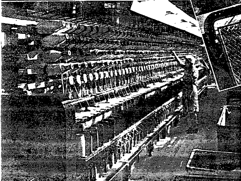
Making Plied Asbestos Yarn on Ring Twisters
