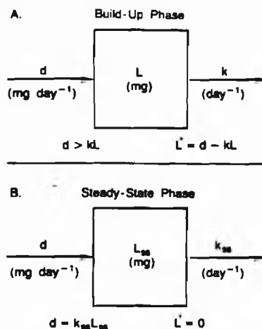
FIG. 1. Build-up and steady-state kinetics of single-compartment lung model employing first-order dust clearance during a chronic dust exposure. (A) The kinetic relationships between dust deposition ( d ) and clearance ( k ) are depicted during the build-up phase of dust in the lungs. The build-up rate is described by L . (B) When the dust burden in the lungs achieves a certain level, the amount of dust removed by first-order clearance ( k_{ss} ) becomes equal to the rate dust deposition ( d ). This heralds the achievement of a steady-state lung burden ( L_{ss} ).
