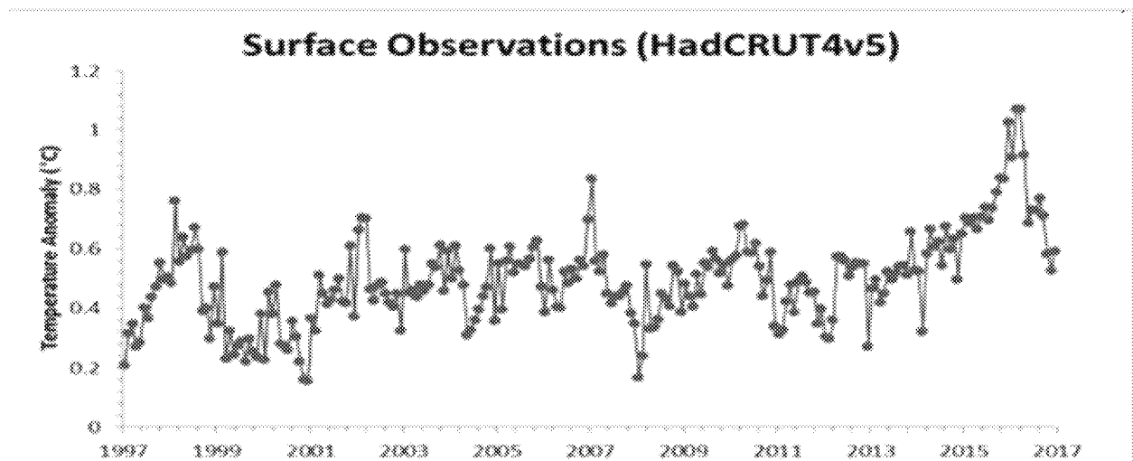
Post-1998 remains controversial. There is a clear "pause" from late 1997 through 2014 (or 2002-2014,
