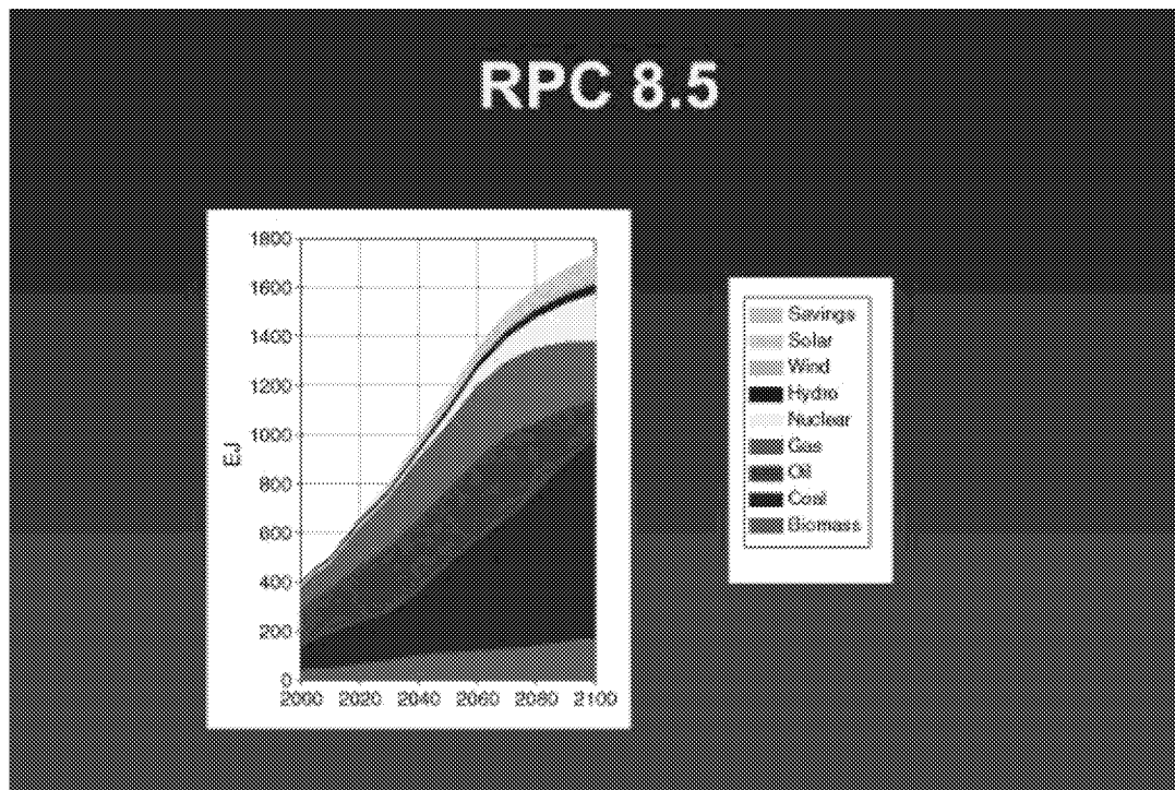
Figure 3. There is no evidence for rapidly increasing displacement of coal with natural gas for electrical generation in RCP 8.5, even though this is now forecast by the IEA worldwide.
