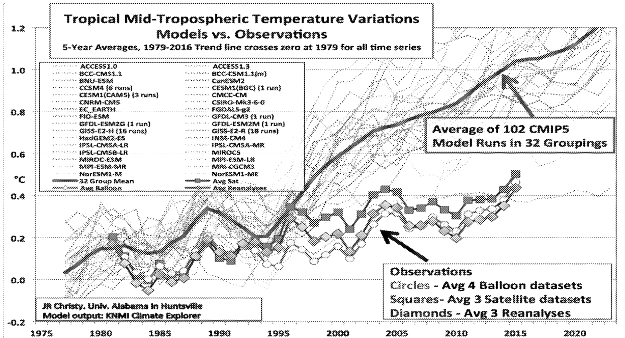
Figure 1. Modelled and observed tropical mid tropospheric (surface-100mb) temperature changes, 1979-2016. From testimony of John Christy to the House Committee on Science, Space and Technology, March 29, 2017. The one model that tracks the observations is INM-CM4. The data are also available in tabular form in the American Meteorological Society's "State of the Climate" report for 2016 (endnote 10).
