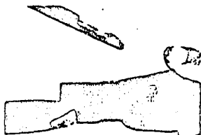
Test sample of aluminum, 3/4 in. long by 1/2 in. wide by 1/16 in. thick, bonded to tire tread rubber 1/2 in. thick, by the Reamite Process. In this test, a pull of 14 lbs. was required to pull the metal strip away from the rubber.
