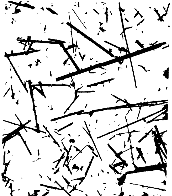
FIG. 2.—Electronmicrograph of UICC eriondite ( \times 1875 ).
