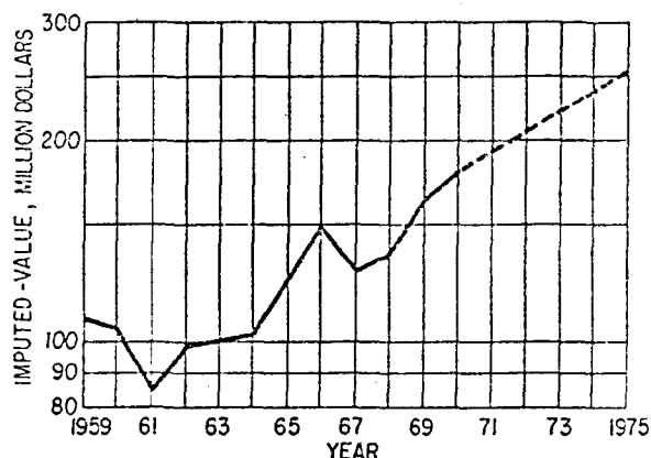
Fig. 6-10—Value of U.S. VCM production, authors' estimates and U.S. Tariff Commission.
