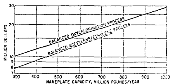
Fig. 6-11—Estimated battery limit capital cost for VCM processes. 14
