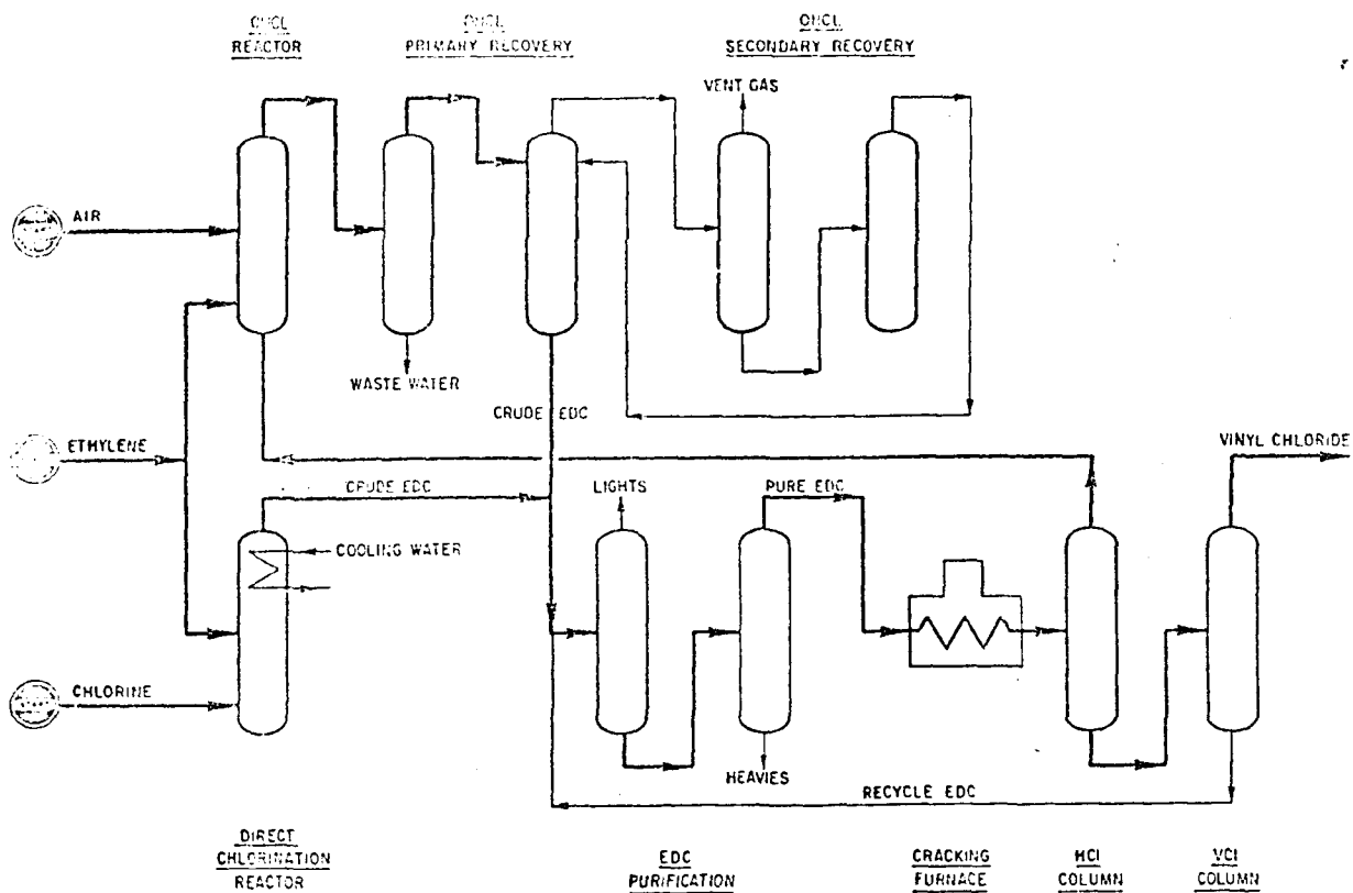
Fig. 6-2—Vinyl chloride by oxychlorination by B.F. Goodrich.
