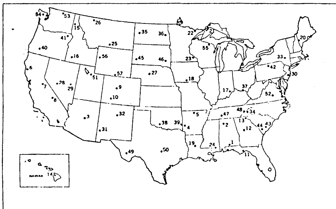
Figure 2.—Map showing location of hydrologic bench-mark stations. Numbers refer to list in Cobb and Biessecker (1971).
