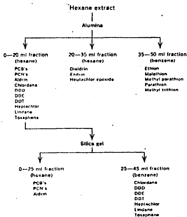
Figure 1.—Scheme for separating polychlorinated biphenyls (PCB's) and polychlorinated naphthalenes (PCN's) from pesticides.
