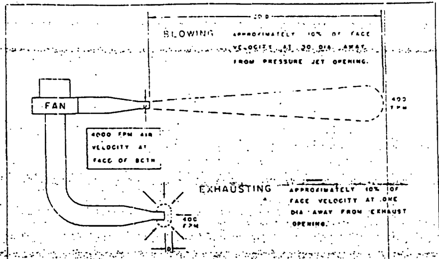
Figure 4. Effect of air blowing OUT of a pipe is felt many feet away, but an exhaust pipe has no effect beyond a few inches from pipe end. Thus it cannot "pick up" material unless pipe and hood are close to the dust source. [Courtesy "Industrial Ventilation—A Manual of Recommended Practice."]
