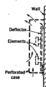
FIG. 2. CONVECTOR HEATER
