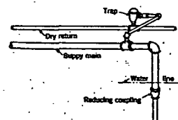
FIG. 40. DRIPPING END OF MAIN INTO WET RETURN
