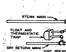
FIG. 41. DRIPPING END OF STEAM MAIN INTO DRY RETURN
