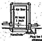
FIG. 36. LOOPING DRY RETURN MAIN AROUND OPENING
