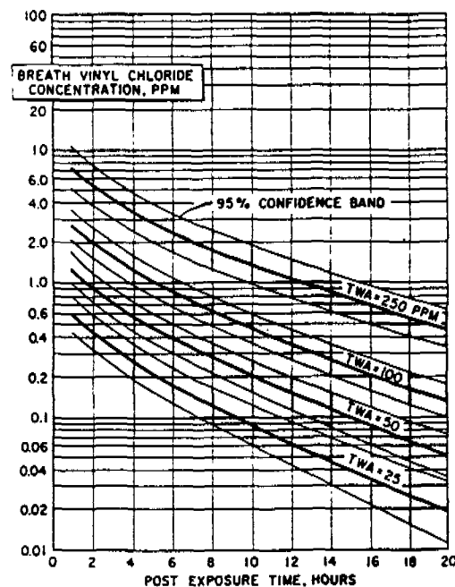
FIGURE 7. Breath decay curves derived from breath data collected from workers following the-job exposures to VCL vapor (8-hour TWA).
