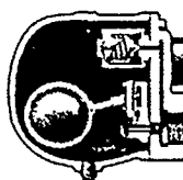
Float Thermostatic
