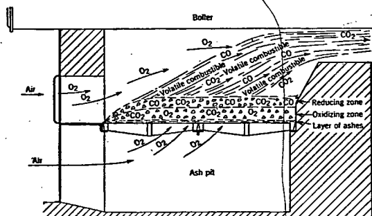
FIG. 1. COMBUSTION OF FUEL IN A HAND-FIRED FURNACE
