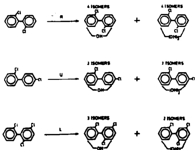
Fig. 1. Metabolism of PCB by Rat Liver Microsomes
