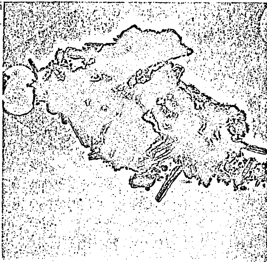
FIG. 7. Electron photomicrograph of air sample taken during brake drum blowing (sac sample No. 4, Table 5). Large numbers (70-100) of chrysotile, some of which are masked by granular particulates, presumably road dust (65,000 total magnification).
