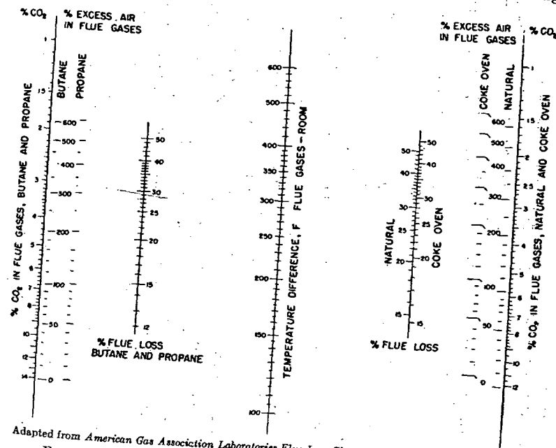
FIG. 7. ALIGNMENT CHART FOR CALCULATION OF FLUE LOSSES FOR BUTANE, PROPANE, COKE OVEN, AND NATURAL GASES
