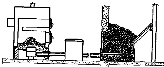
FIG. 6. UNDERFEED STOKER, BIN FEED TYPE, CLASS 1
