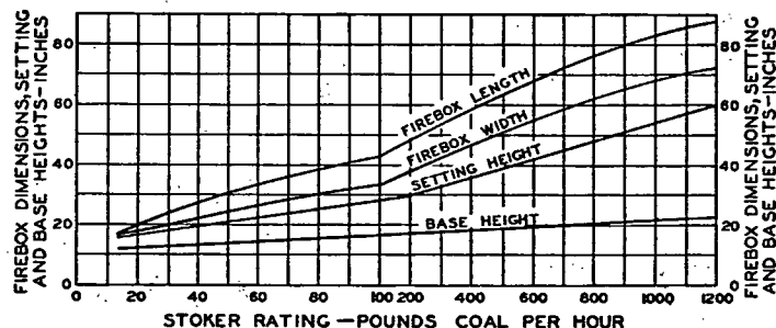
FIG. 11. SUGGESTED MINIMUM FIREBOX DIMENSIONS AND BASE HEIGHTS*
