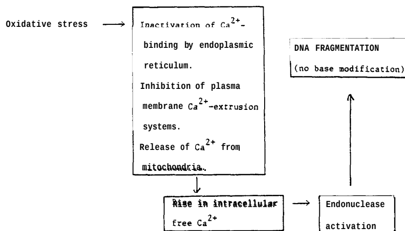
Fig. 1. Hypotheses to explain DNA damage resulting from exposing cells to oxidative stress.
