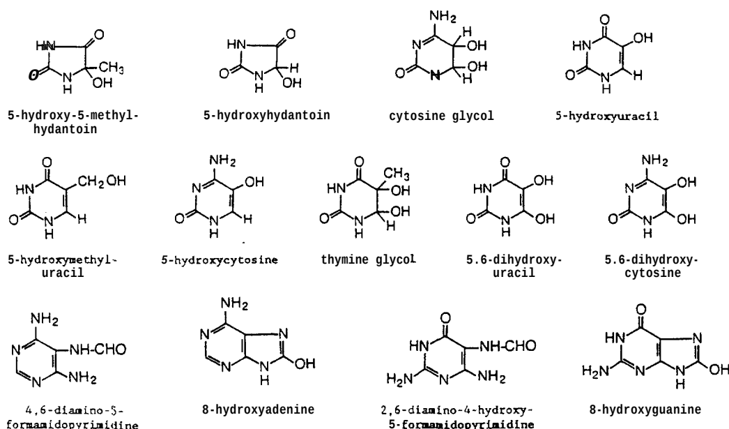
Fig. 4. Some of the end-products that result from attack of hydroxyl radicals upon the bases of DNA.
