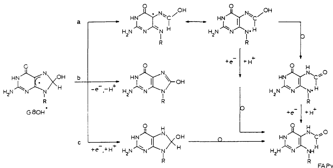
Fig. 3. Some of the products that can result from attack of hydroxyl radicals upon guanine. Adapted with permission from reference [138]. G8OH • is the radical formed by attack of • OH upon C8 of guanine. It can undergo ring opening followed by reduction and protonation to give FapyGua (route a), oxidation to 8-OH-Gua (route b) or reduction to give 7,8-dihydro-8-hydroxyguanine, which can be converted to FapyGua (route c).
