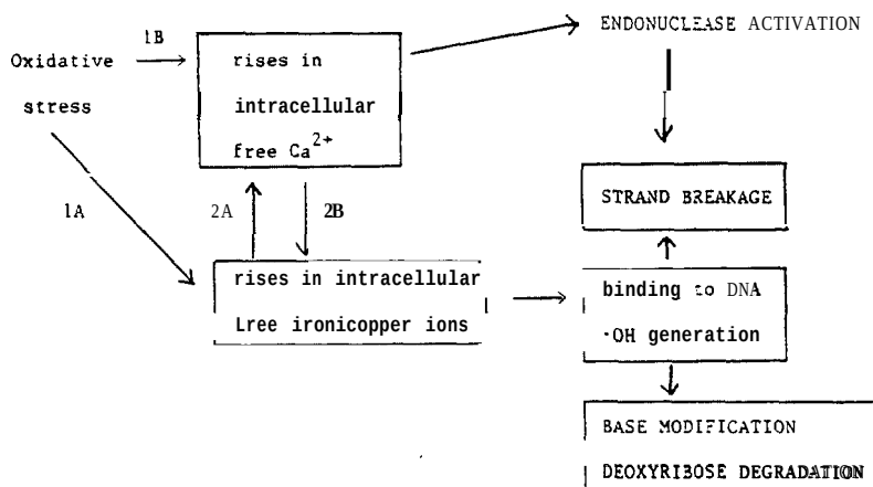
Fig. 2. A combined hypothesis. Rises in intracellular free iron or copper ion concentrations could be a consequence of rises in Ca 2+ (1B, 2B) or vice versa (1A, 2A).
