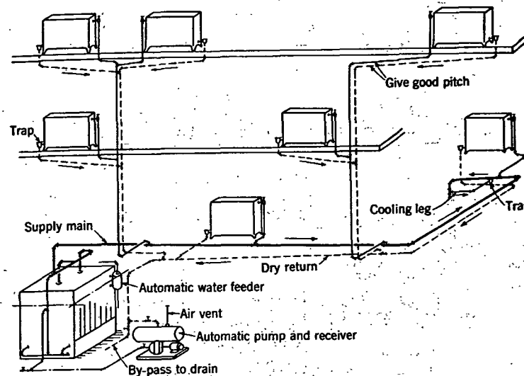
FIG. 11. TYPICAL INSTALLATION USING CONDENSATION PUMP
