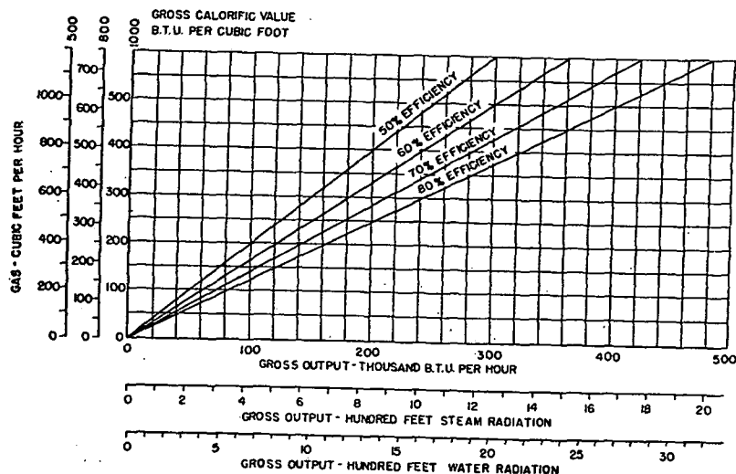
FIG. 3. GAS FUEL BURNING RATE CHART
