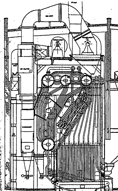
Cross-section of one unit installed at J. I. Case
