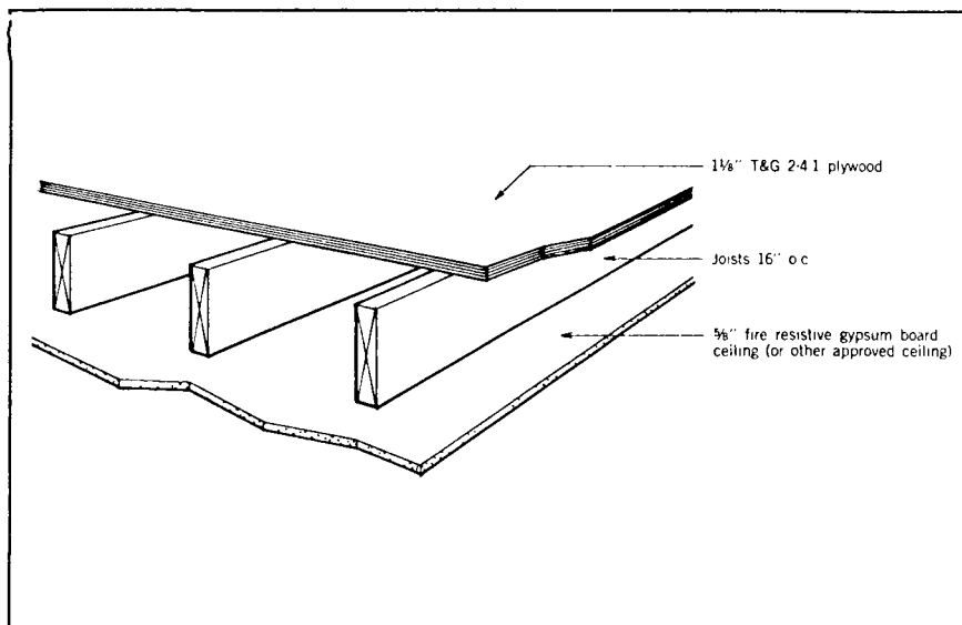
Figure 4. One-hour assembly — 1 \frac{1}{8} " plywood with joists 16" o.c.
