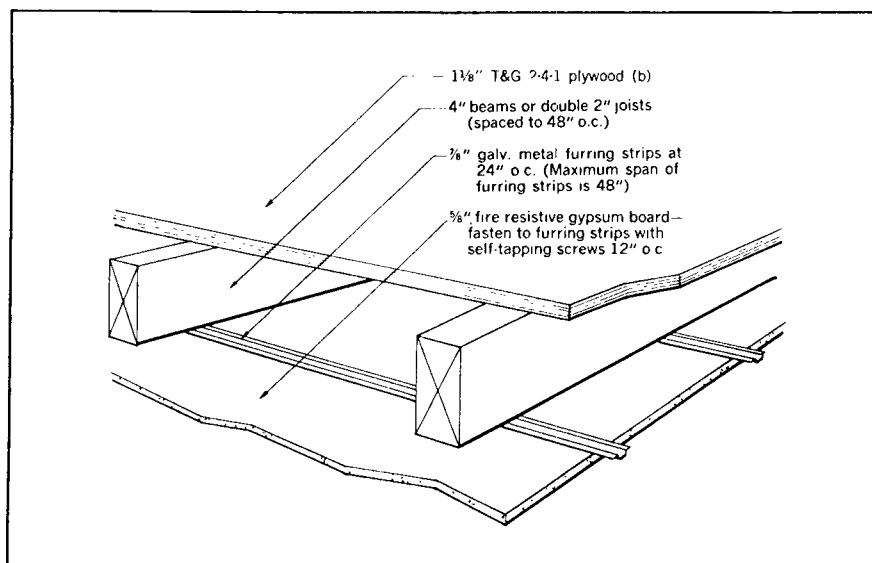
Figure 5. One-hour assembly — 1 \frac{1}{8} " plywood with beams 48" o.c.
