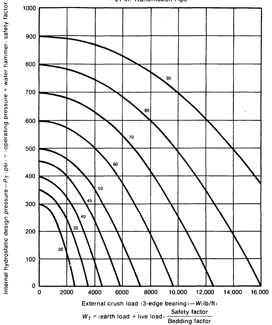
Fig. 14c. 21-in. Transmission Pipe
