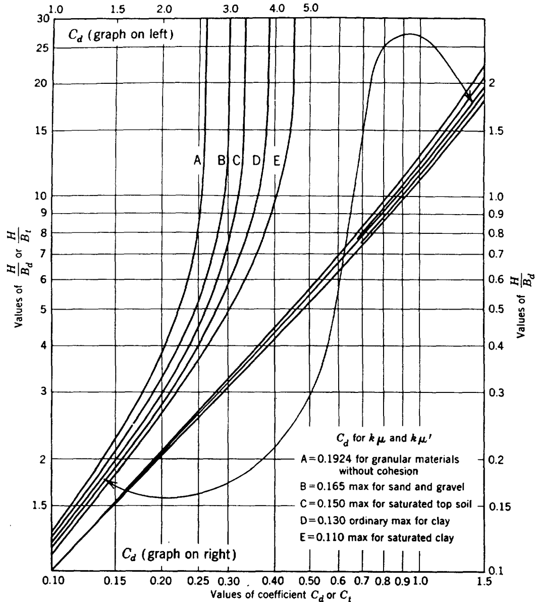
Fig. 5. Values of C_d for Trench Conditions
