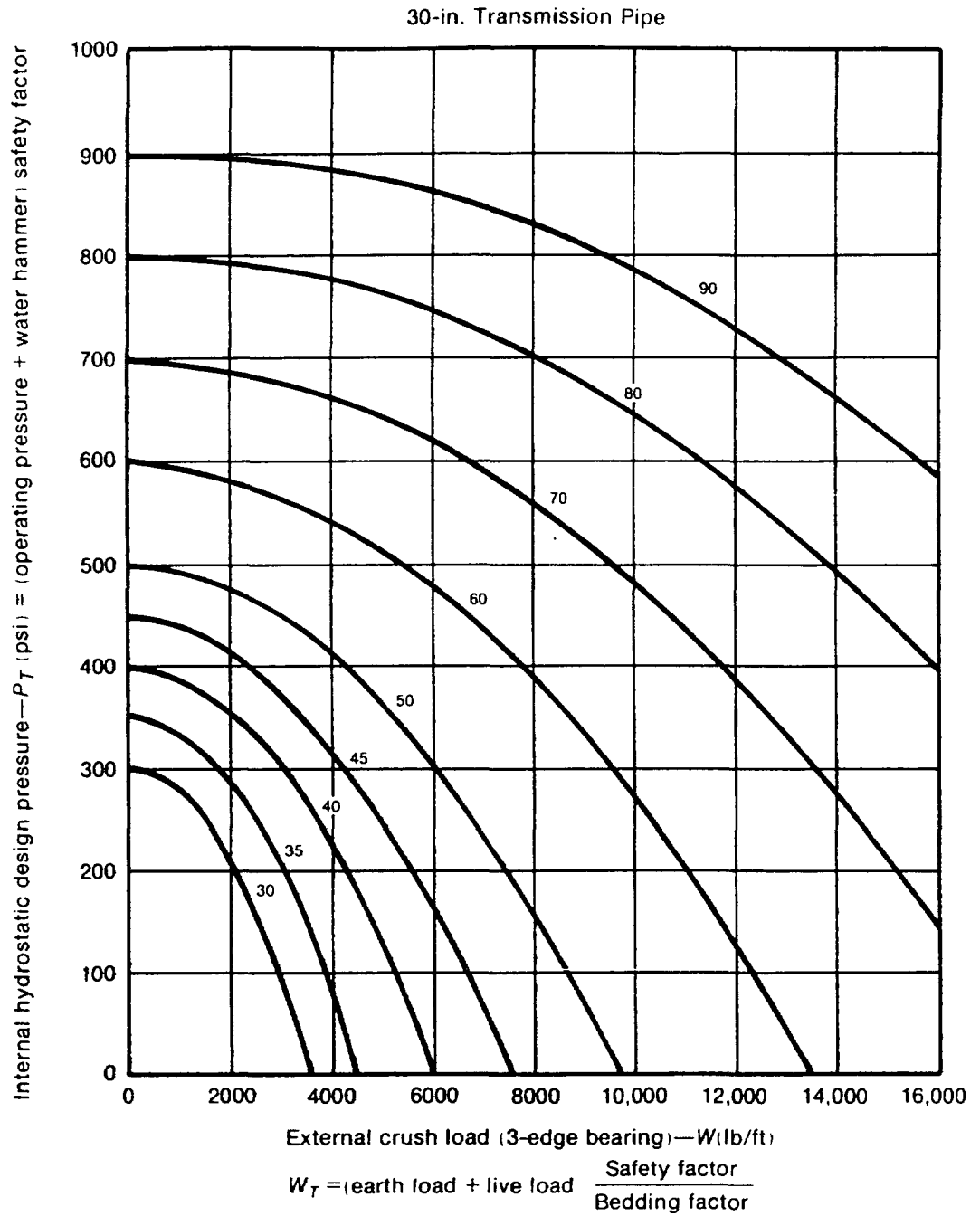
Fig. 14f. 30-in. Transmission Pipe
