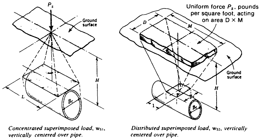
Fig. 13. Superimposed Loads
