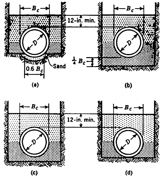
Fig. 1. Bedding Conditions
