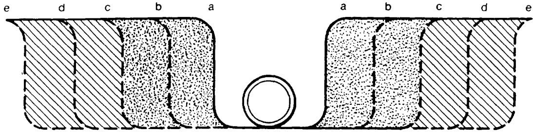
Fig. 6. Embankment Conditions
