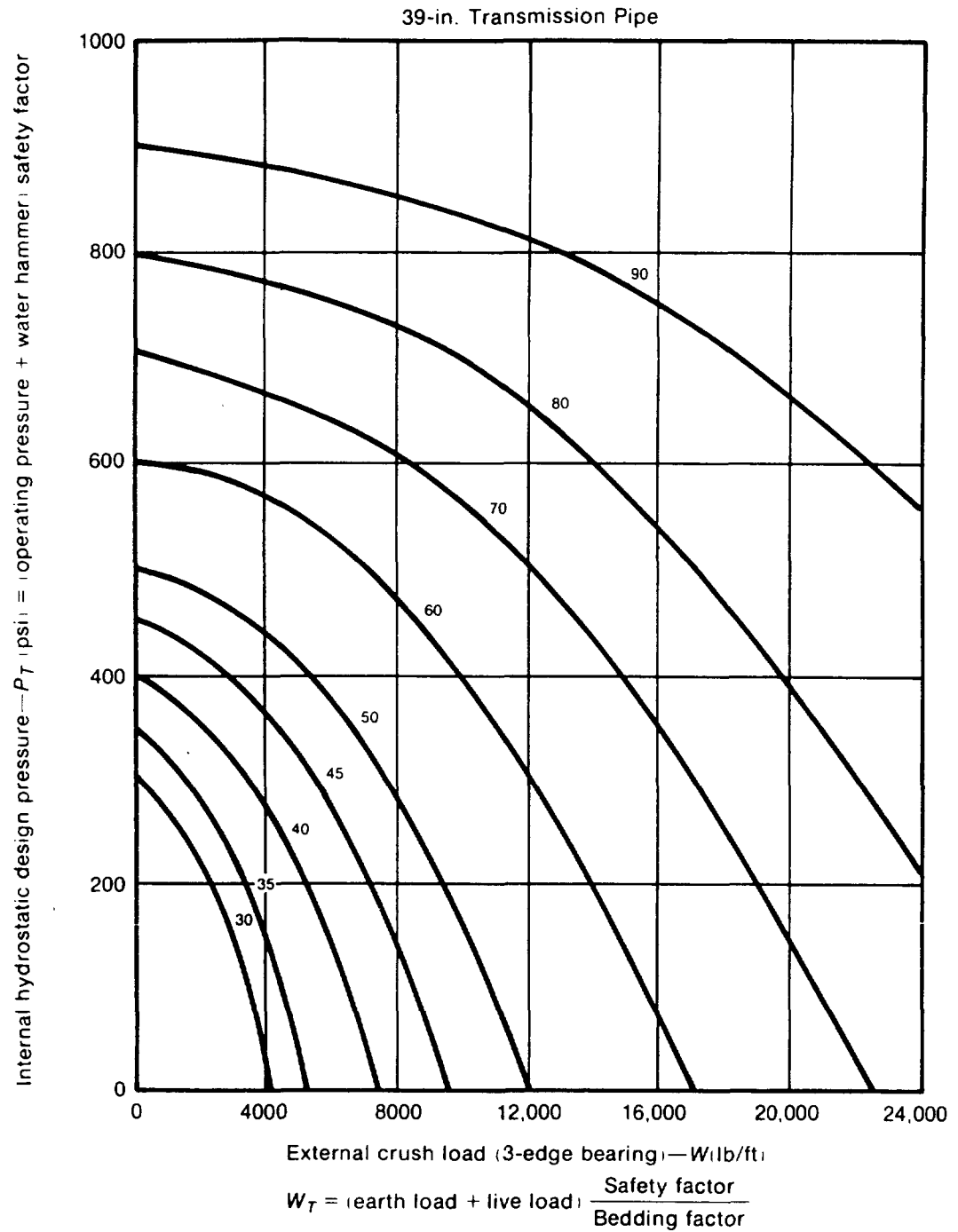
Fig. 14i. 39-in. Transmission Pipe
