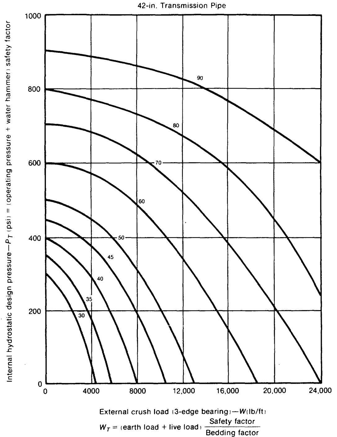
Fig. 14j—42-in. Transmission Pipe
