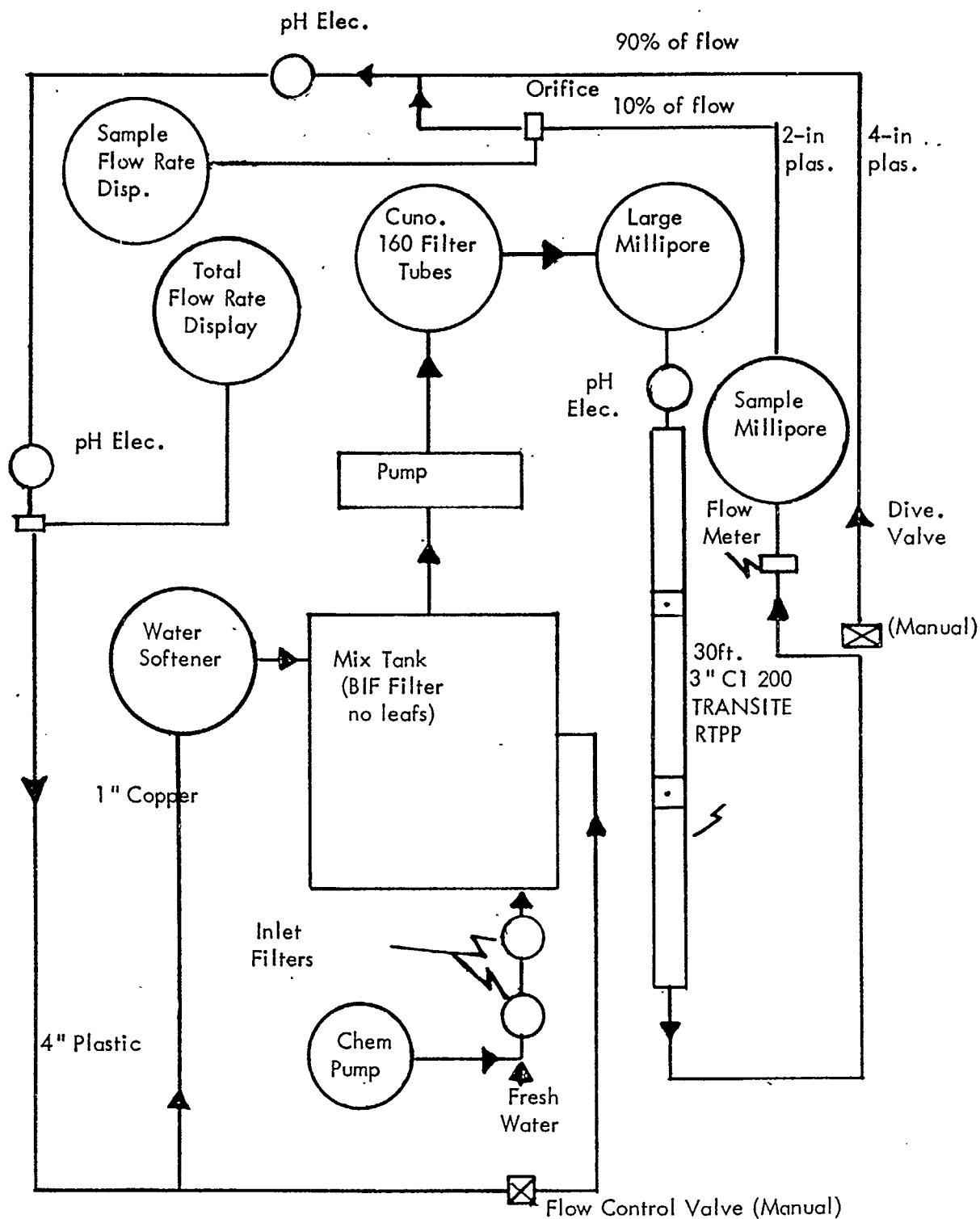
Figure 1. Schematic Diagram of Test Line Installation
