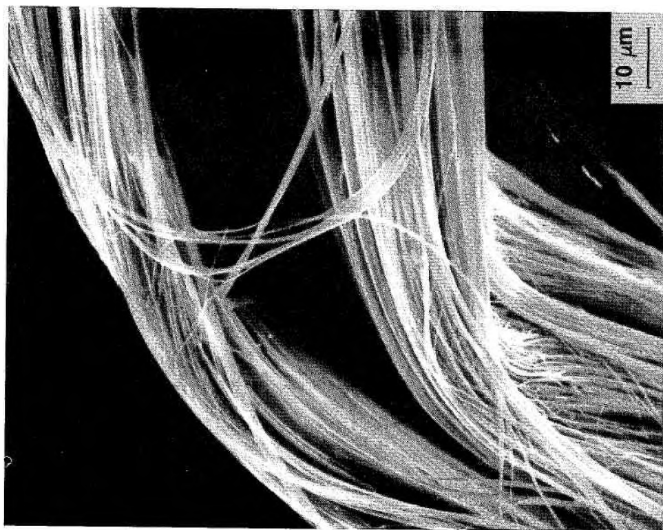
FIG. 2. Scanning electron-micrograph of a potassian winchite fibre.
