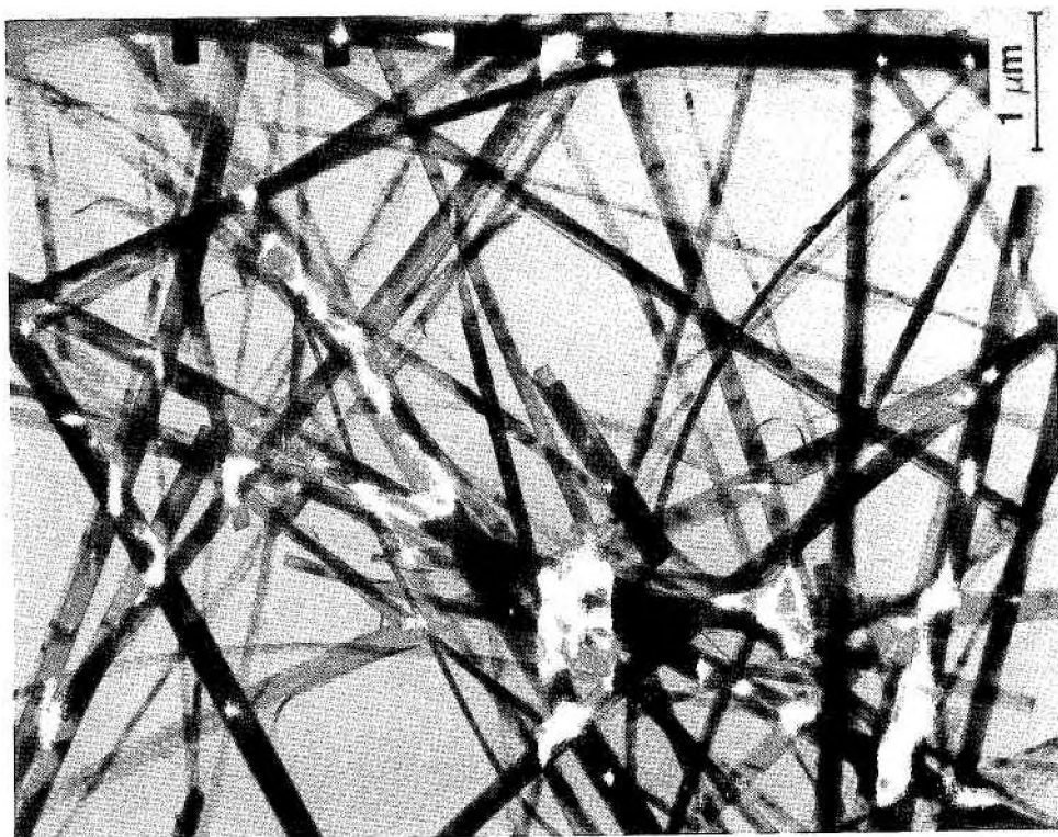
FIG. 3. Transmission electron-micrograph showing potassian winchite fibrils. The ribbon-shaped fibrils are between 200 and 400 Å in cross-section. Some are slightly wrinkled, and some portions appear as dark streaks because they are in the correct position to produce Bragg reflections.
