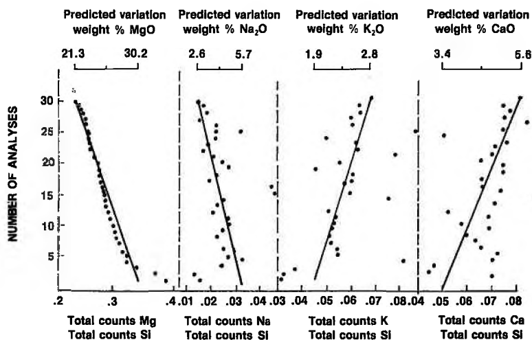
FIG. 5. Summary of the variations in peak area (element)/peak area(Si) determined in 30 analyses of potassian winchite-asbestos by a scanning electron-microscope equipped with an energy-dispersive X-ray spectrometer. From the spectrograph, total peak-areas of Mg, Na, K and Ca are compared to total peak-area of Si. The variations in weight percent of the oxides MgO, Na 2 O, K 2 O and CaO, as predicted from the spectrometer data, are indicated.
