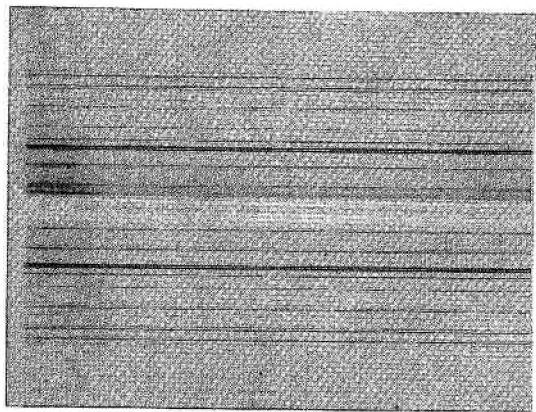
FIG. 1. Zero-level Weissenberg photograph of a potassian winchite fibre. The axis of rotation of the fibre is the c crystallographic axis. Ni filtered Cu radiation, 30 kV, 20 mA.
