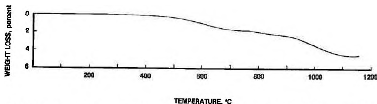
FIG. 4. TGA tracing of potassian winchite-asbestos. Heating rate was 5^{\circ} per minute. The analysis was performed in a N_2 atmosphere.
