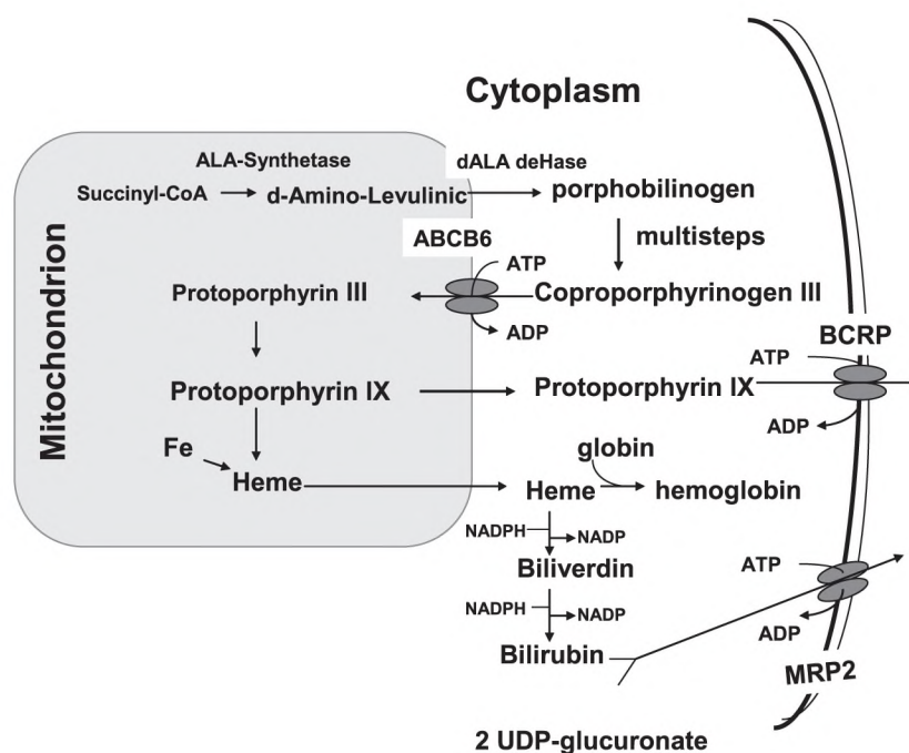
FIG. 11. Metabolic pathways of heme/porphyrin biosynthesis and elimination by ABCG2 transporter
